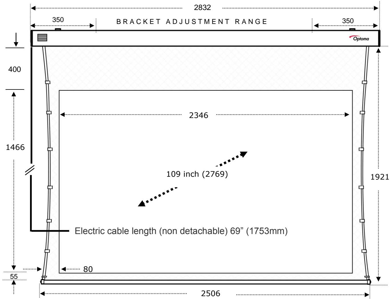
Optoma 16:10 DE-1109ETT ELECTRIC SCREEN Measurements in Milimetres
