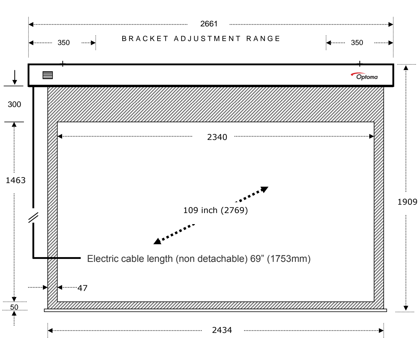
Optoma 16:10 DE-1109EGA ELECTRIC Measurements in Milimetres
